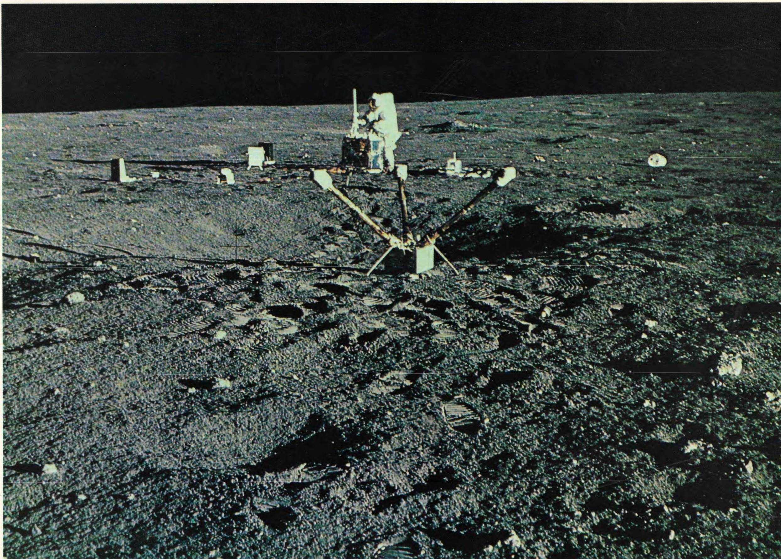
DEPLOYING THE APOLLO LUNAR SURFACE EXPERIMENTS PACKAGE (ALSEP), APOLLO 12. Instruments measure the solar wind; pressure, temperature, and composition of atmosphere; the magnetic field at the lunar surface; and seismic activity.
