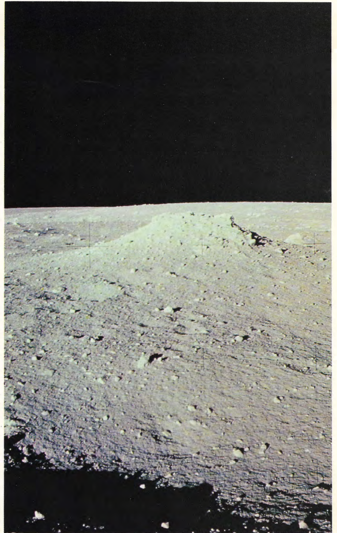
A MOUND ON THE LUNAR SURFACE, one of two observed by the Apollo 12 astronauts. There is no explanation yet for this feature.
