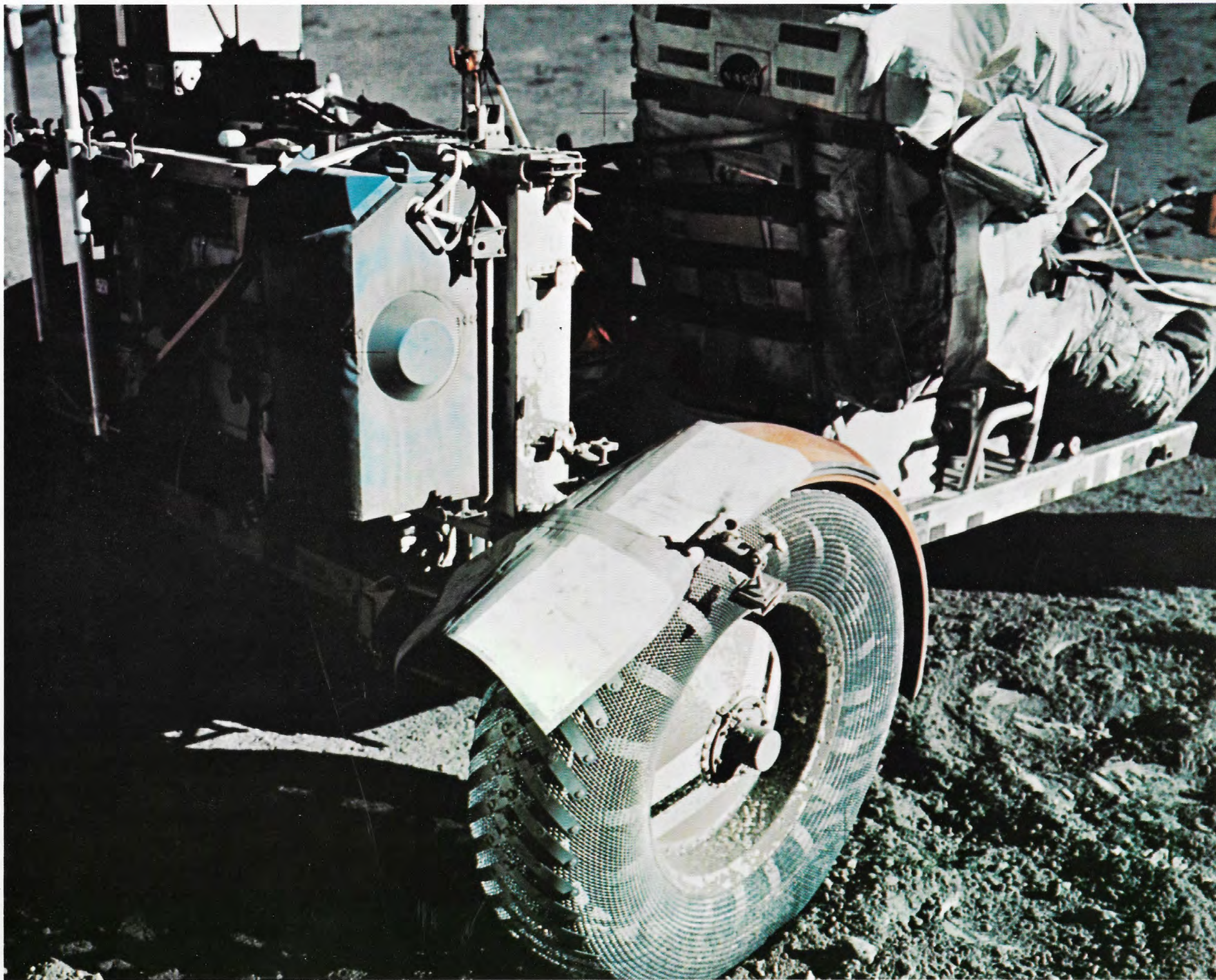
APOLLO 17 – Makeshift repair on the fender of the Lunar Roving Vehicle.
