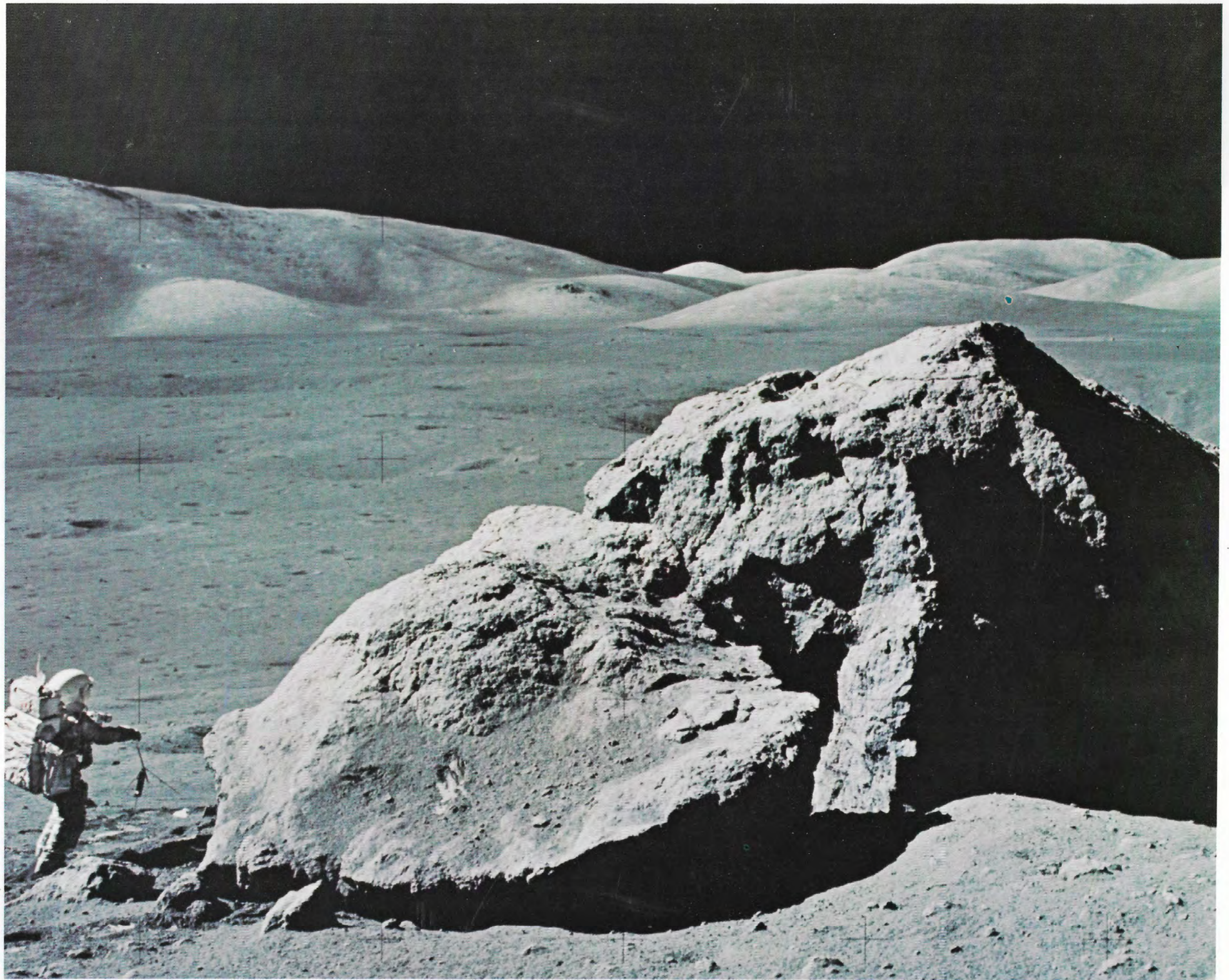
APOLLO 17—A huge, split lunar boulder at the Taurus-Littrow landing site.
