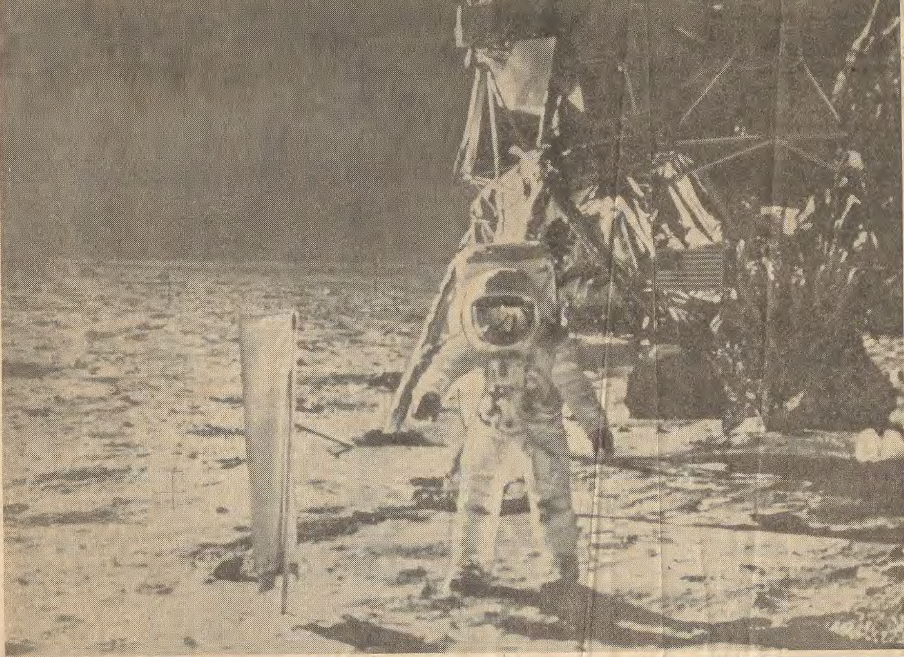
● Aldrin approaching the solar wind collector, which consisted of a sheet of aluminium foil. The foil, which collected atomic particles driven by the solar wind, was brought back to earth by the lunarnauts
