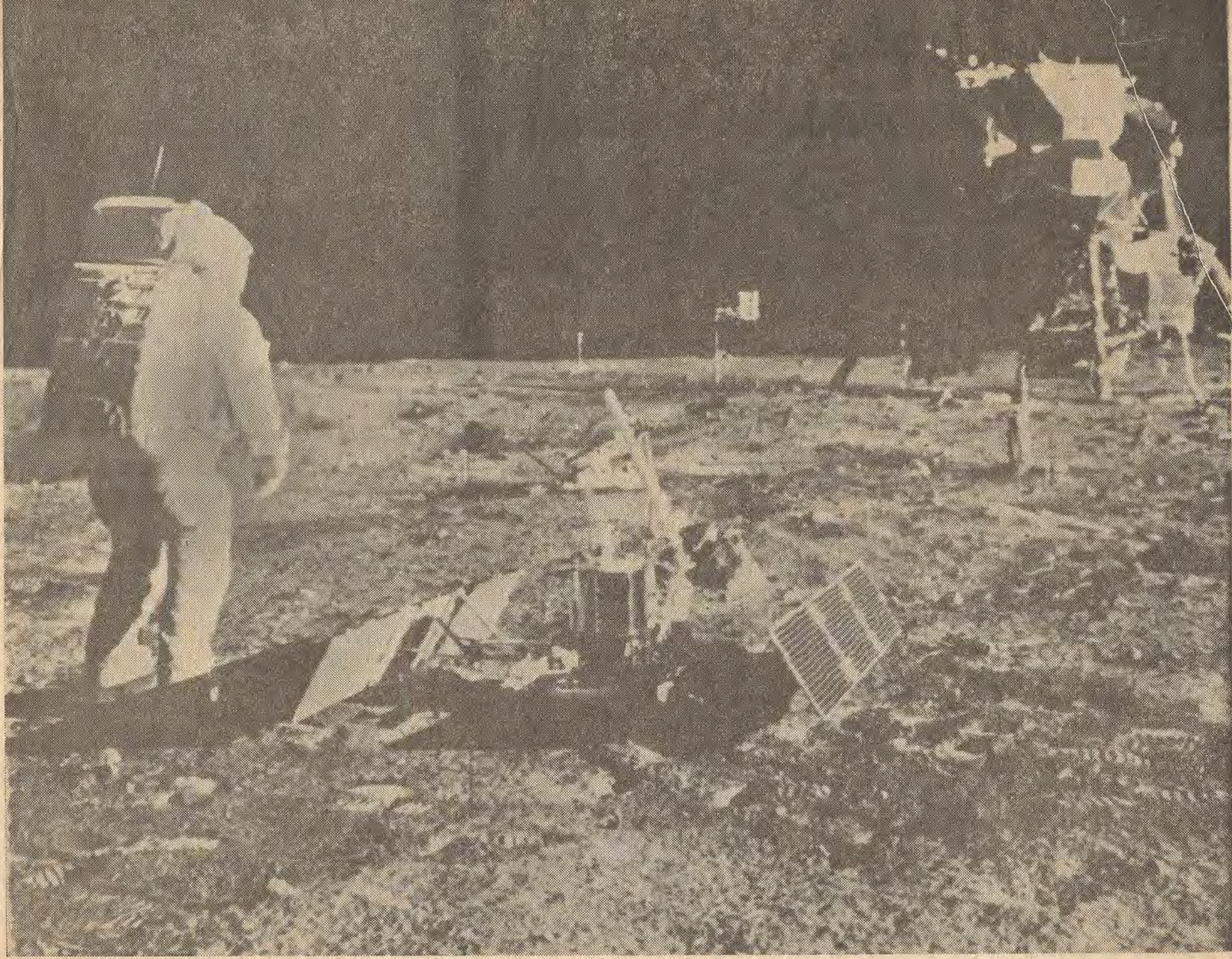
● Col Edwin Aldrin standing beside the massive seismometer, which they left on the lunar surface to record moonquakes. Immediately behind it is the mirror to reflect laser light beams from earth and in the background, beside the module, are the American flag and the small television camera.
