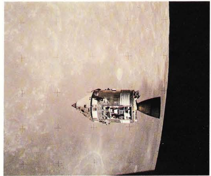
Endeavour (Apollo 15 command/service module) in lunar orbit. SIM (Scientific Instrument Module) bay is exposed.
